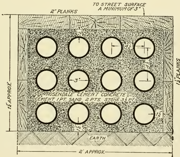
Fig. 46. Cross-Section of Wrought-Iron Pipe Conduit
